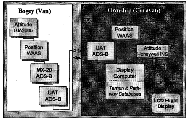
Figure 4. Runway Incursion Alerting System - Block Diagram
